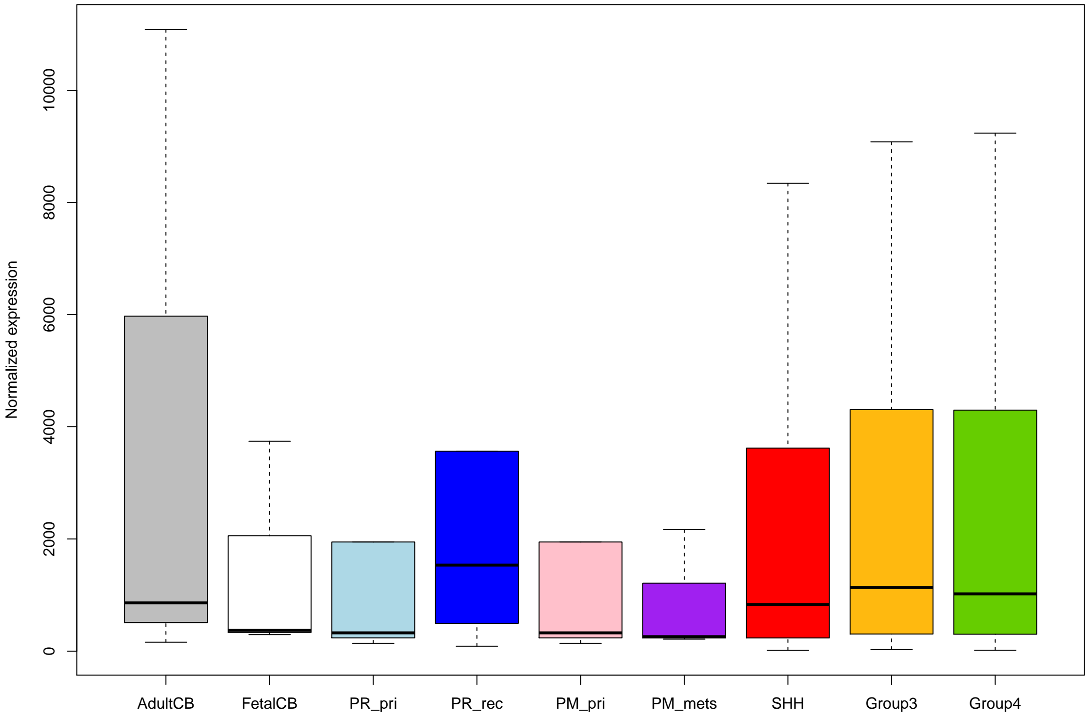
ENSG00000064687_ABCA7_+ expression (no outliers)
