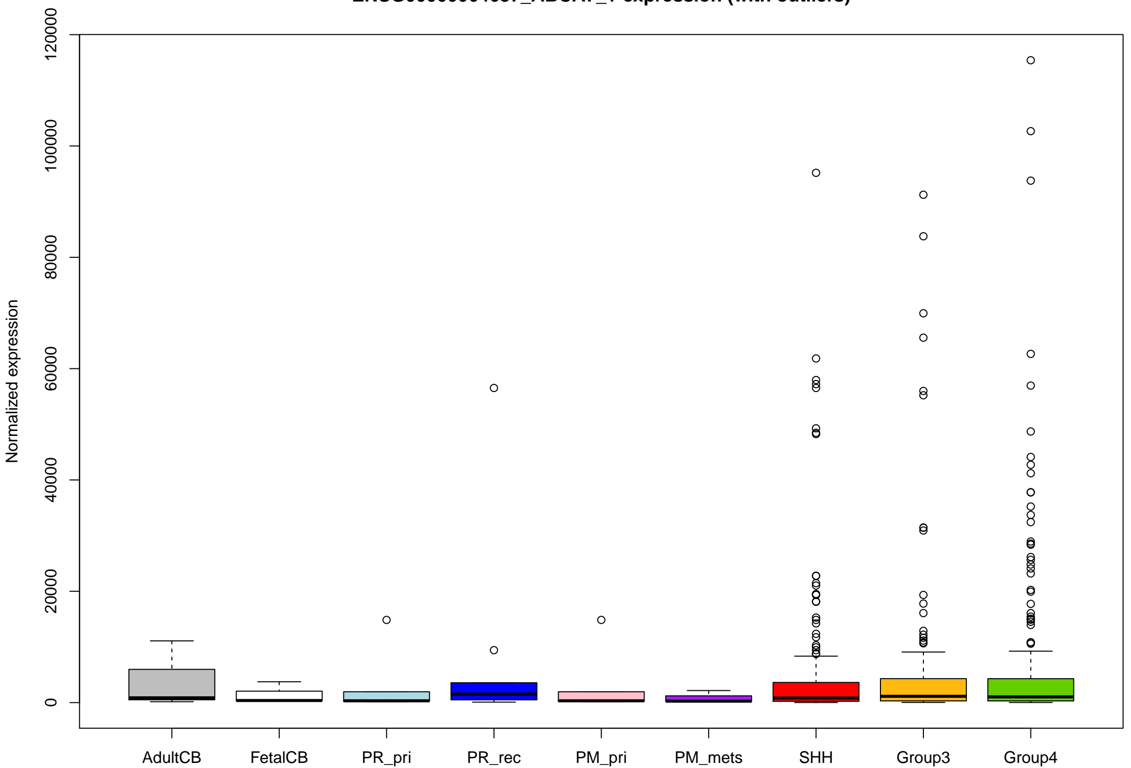
ENSG00000064687_ABCA7_+ expression (with outliers)
