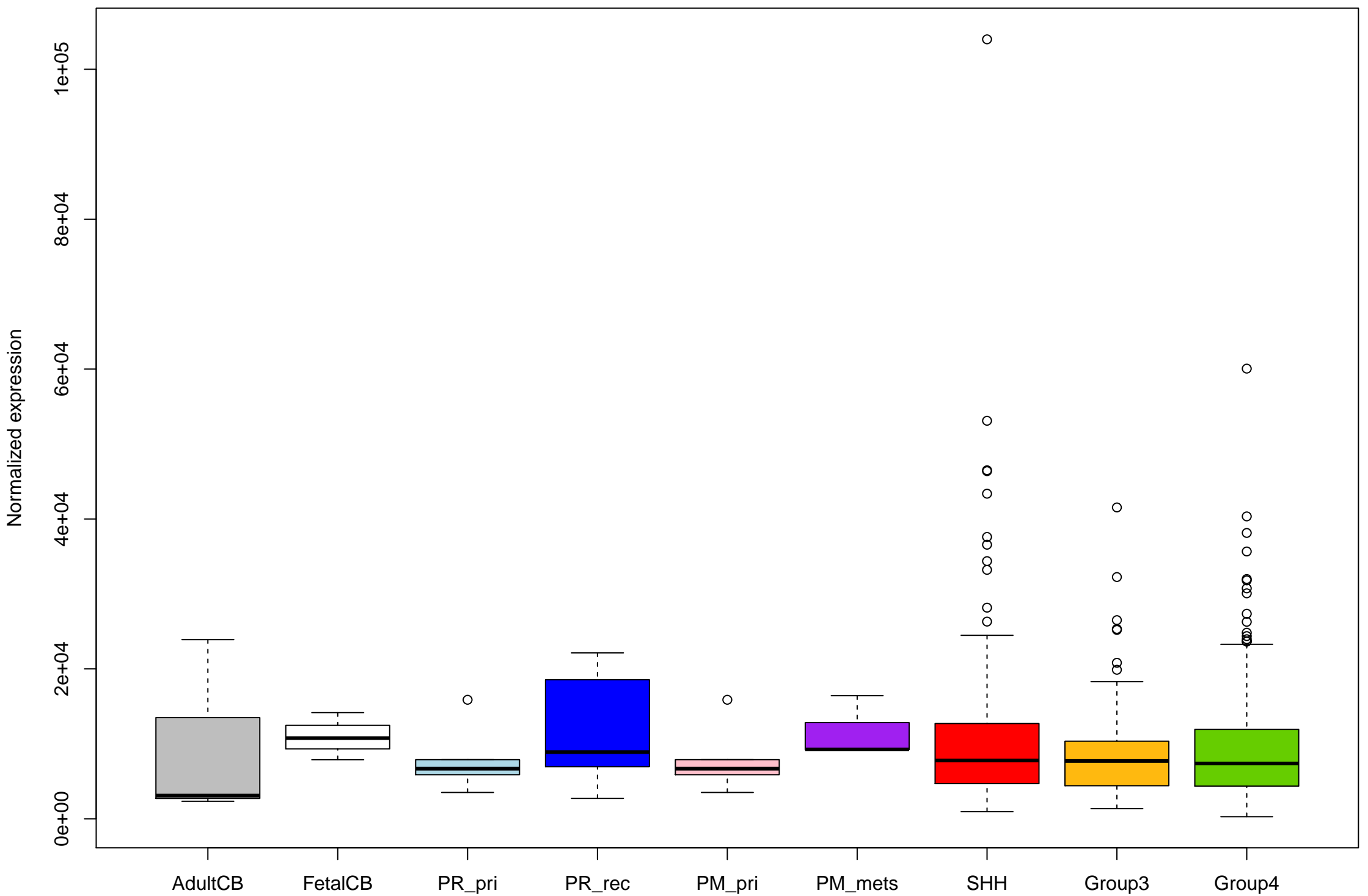
ENSG00000136068_FLNB_+ expression (with outliers)
