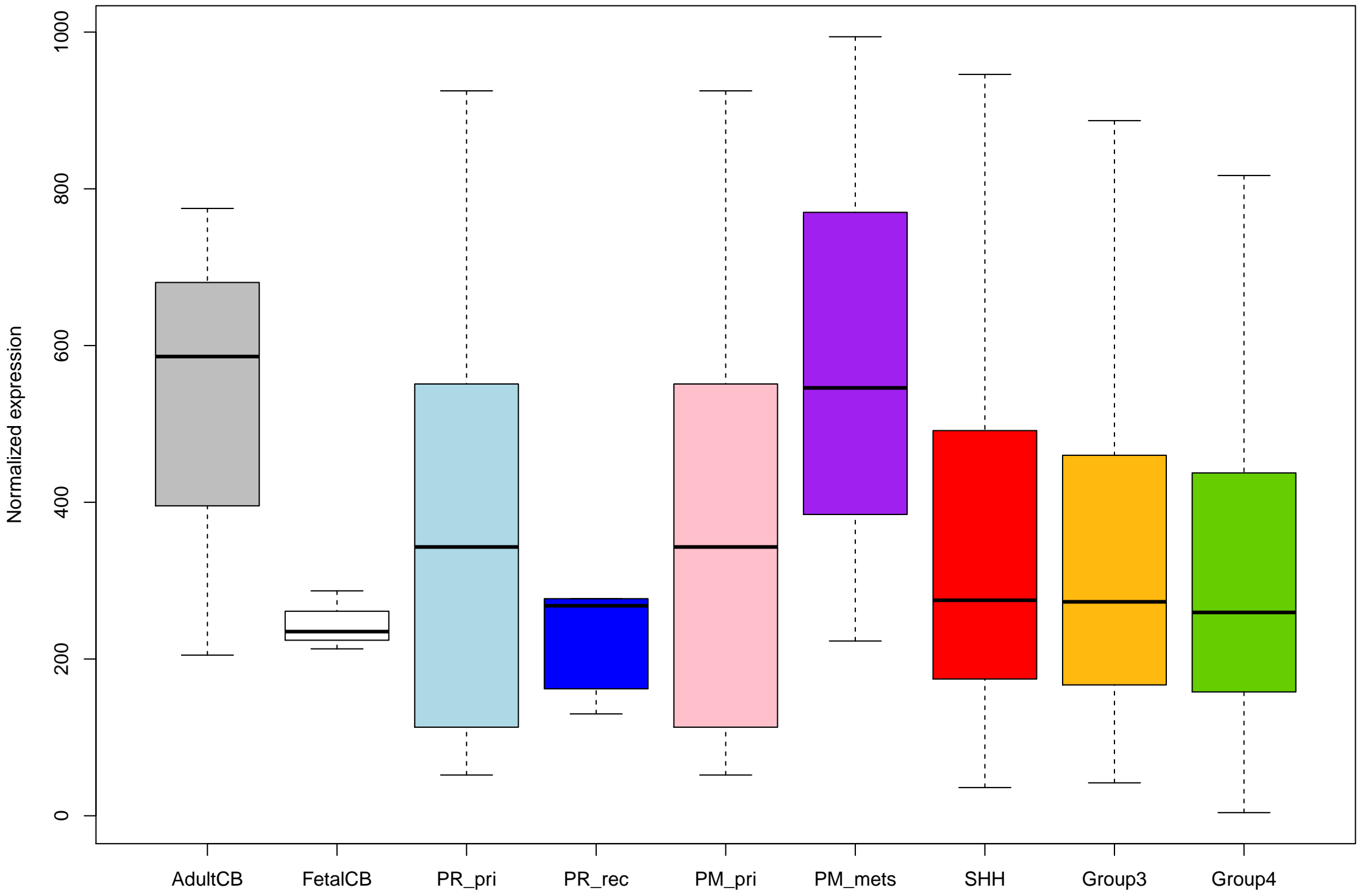
ENSG00000152049_KCNE4_+ expression (no outliers)
