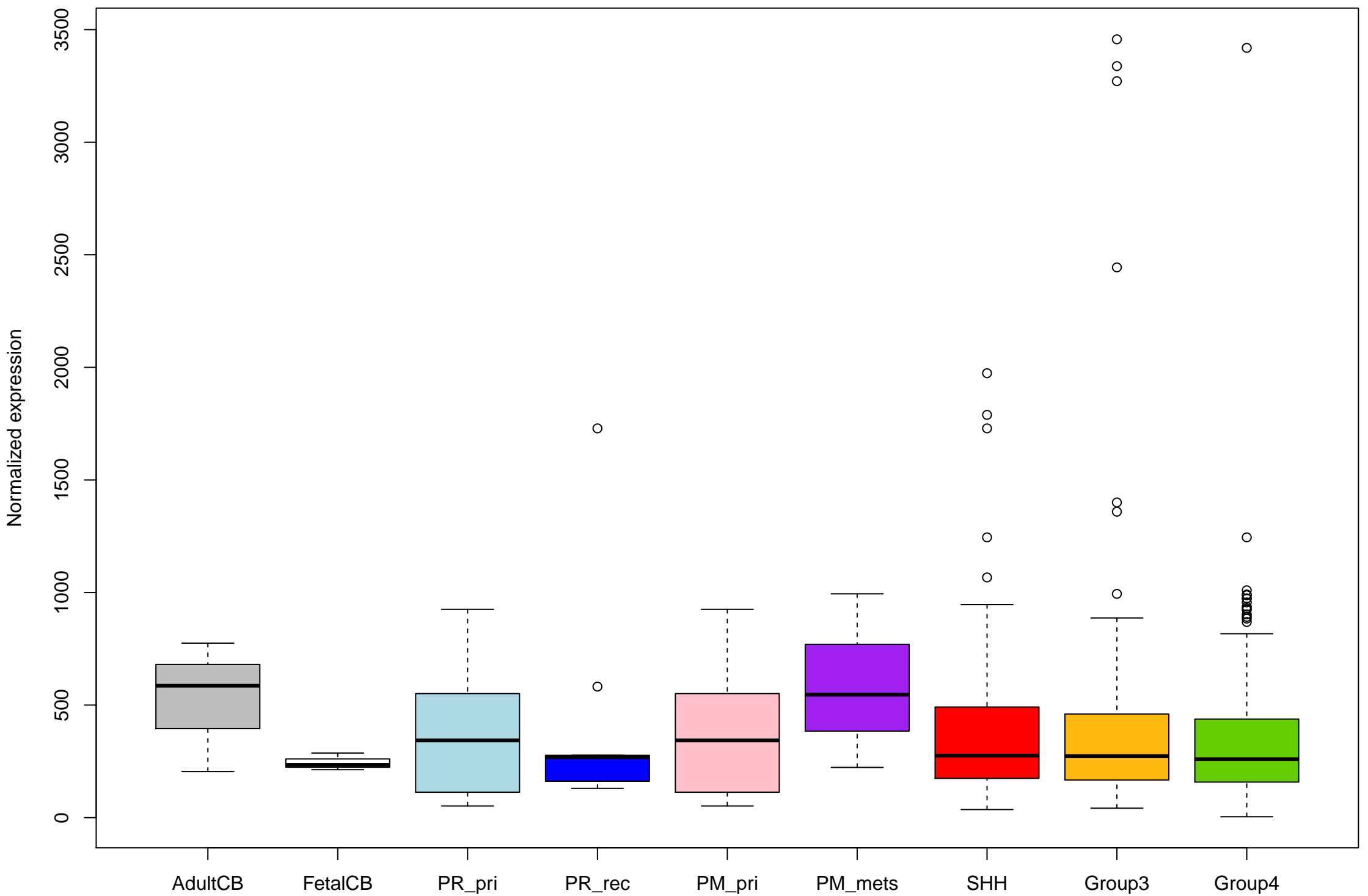
ENSG00000152049_KCNE4_+ expression (with outliers)
