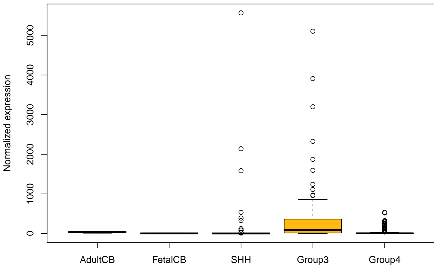
CD70 ENSG00000125726 expression (including outliers)
