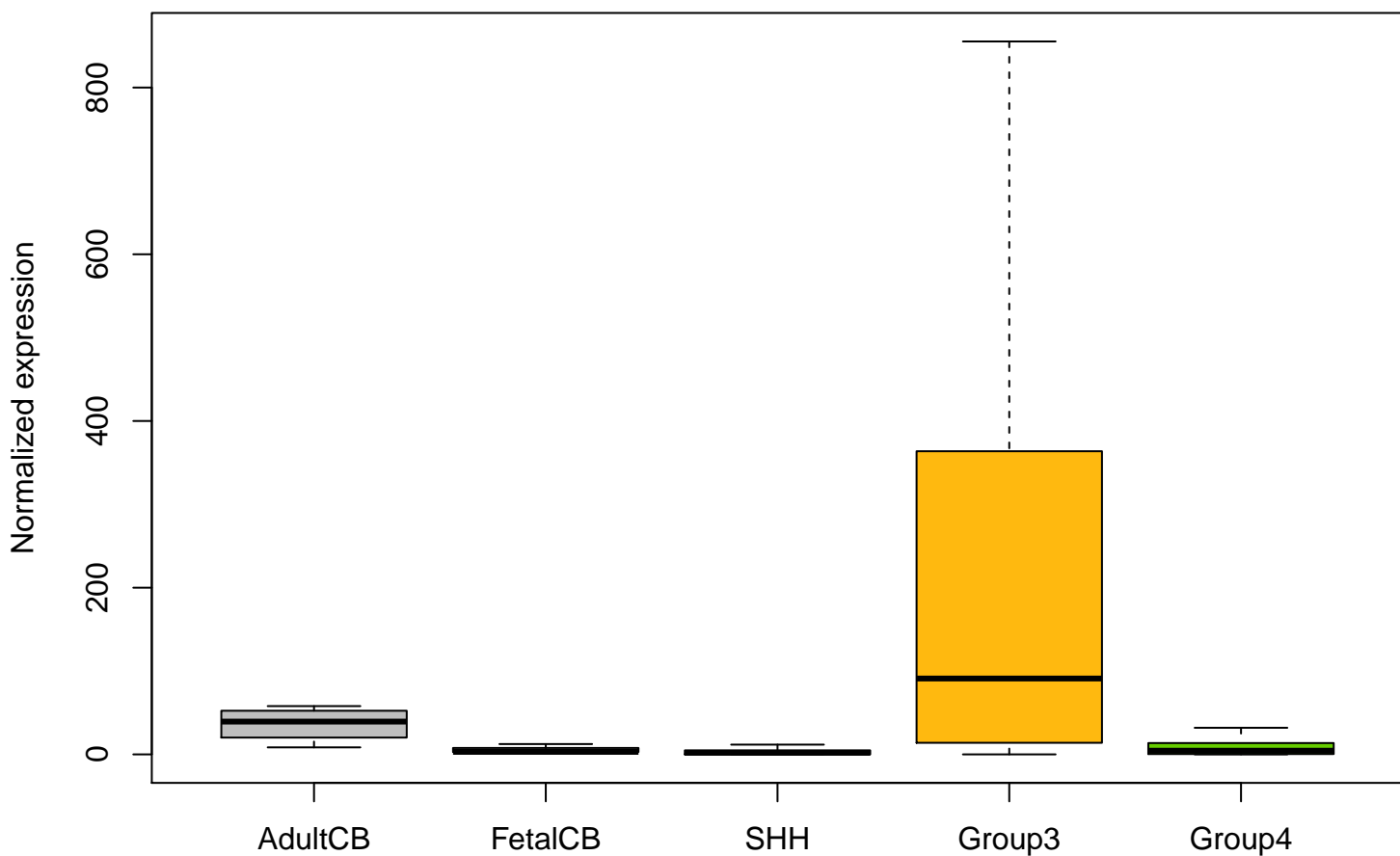
CD70 ENSG00000125726 expression (no outliers)
