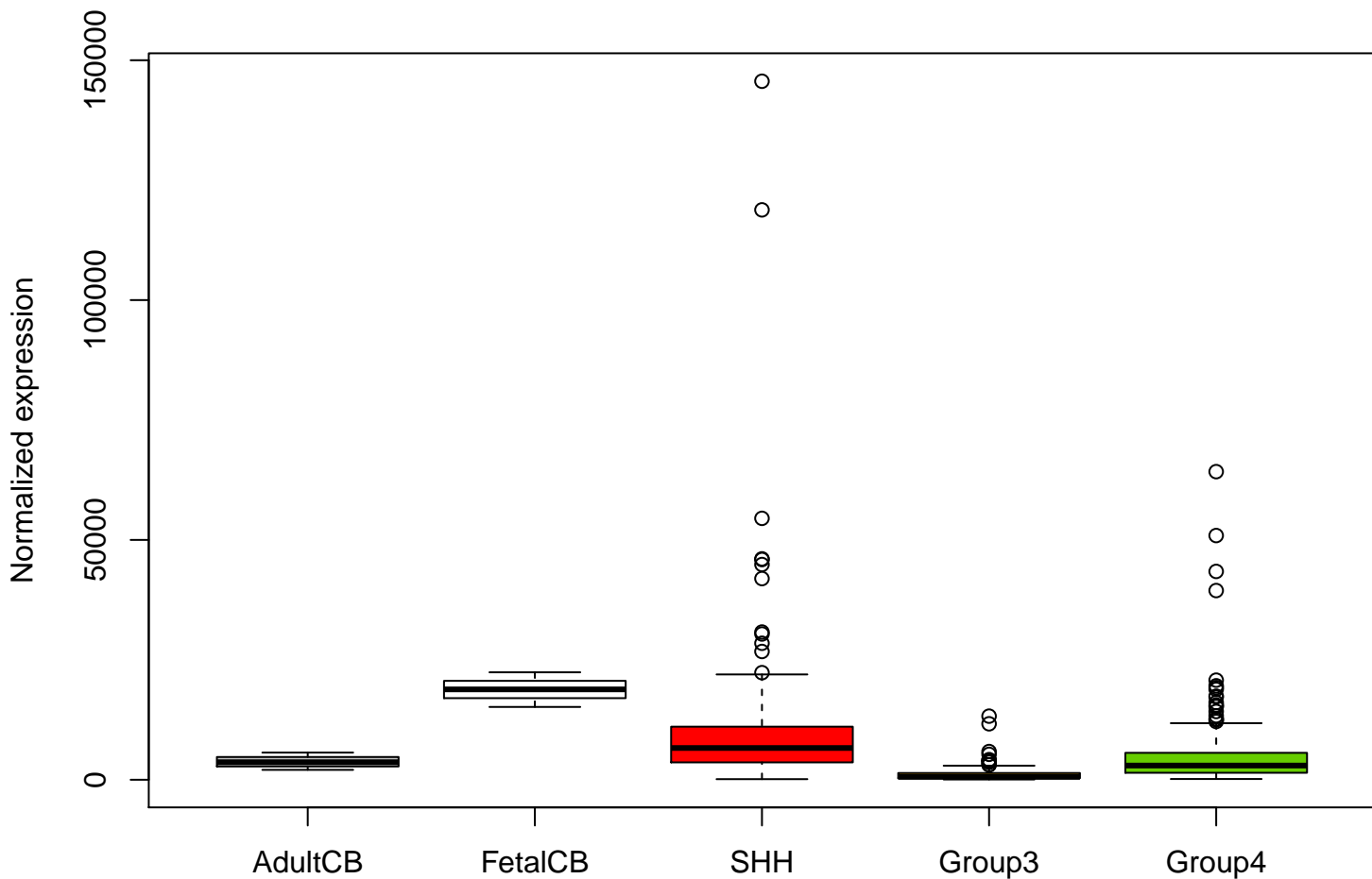
EGFR ENSG00000146648 expression (including outliers)
