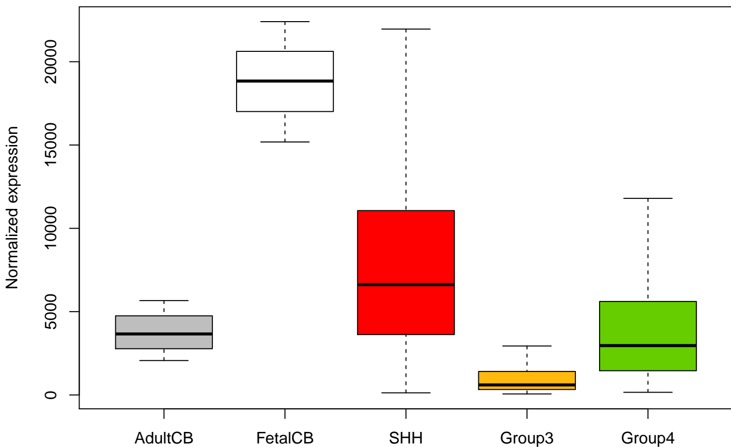
EGFR ENSG00000146648 expression (no outliers)
