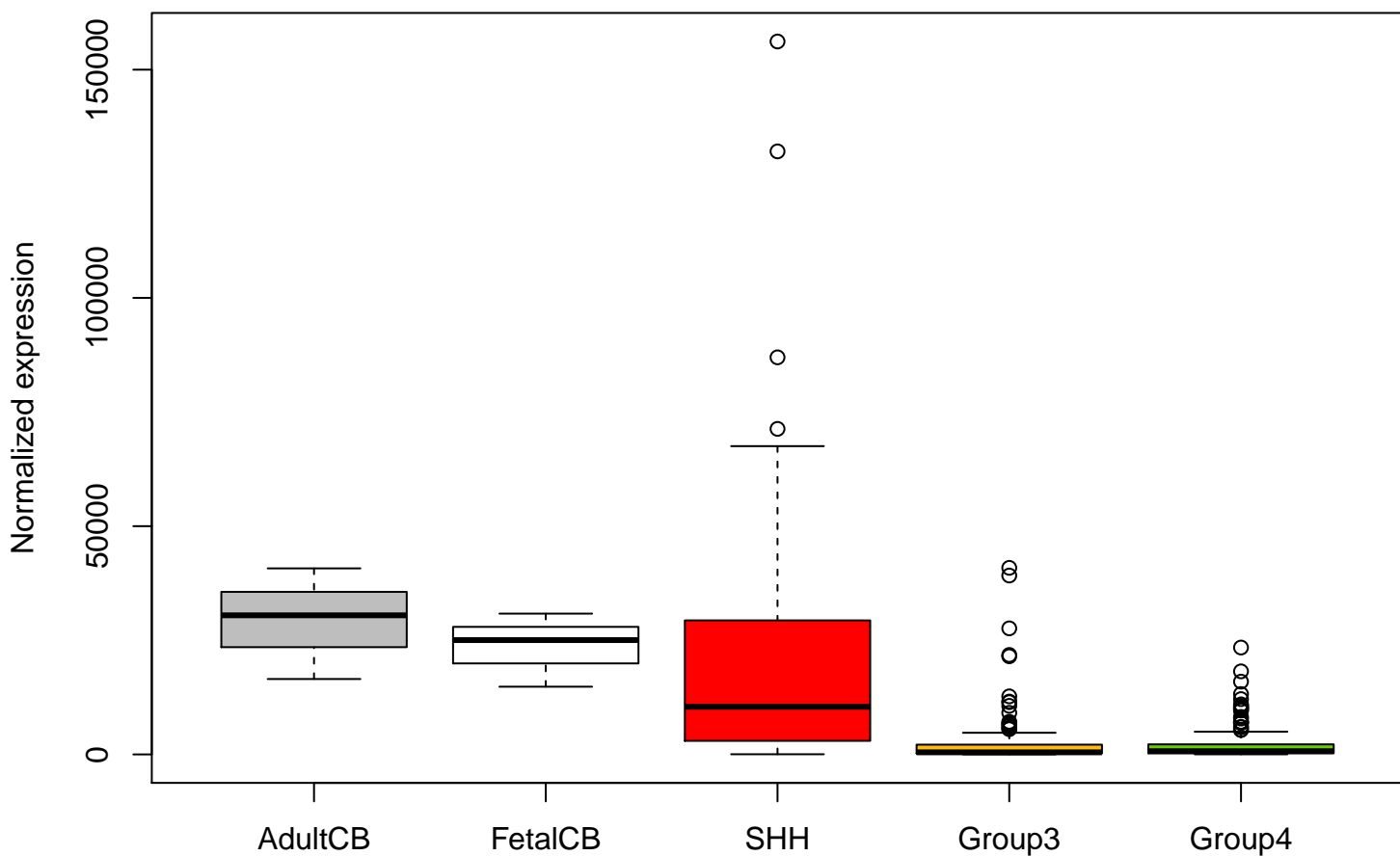
CNTN2 ENSG00000184144 expression (including outliers)
