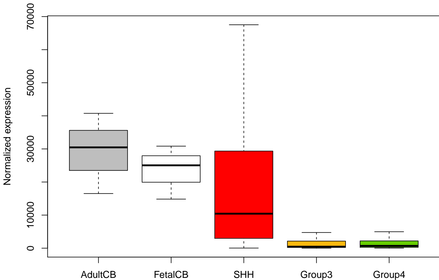
CNTN2 ENSG00000184144 expression (no outliers)
